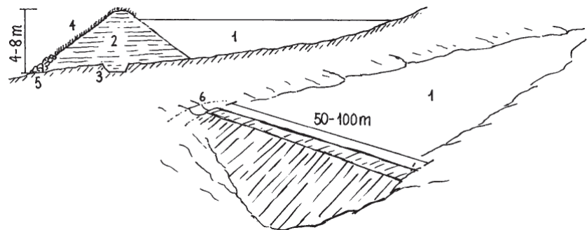
Dimensions and main components of a small dam: (1) water body; (2) dam wall (with layers of compacted soil; side slopes, 3:1); (3) central core ('key'); (4) grass cover; (5) stone apron; (6) spillway. Source: Liniger, H.P., et al. (2011).
